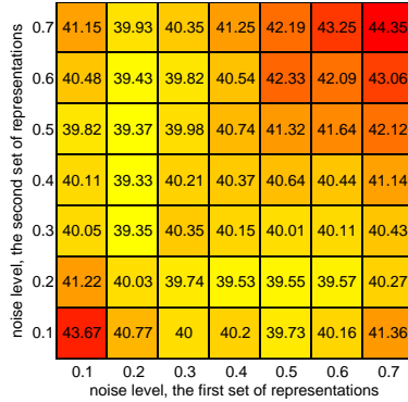
Figure 5: Test errors yielded by representations constructed by concatenating representations learnt with various levels of noise. This allows representations that are otherwise weak separately to achieve low test errors, e.g. for \nu = 0.1 and \nu = 0.5 (cf. Figure 1).
