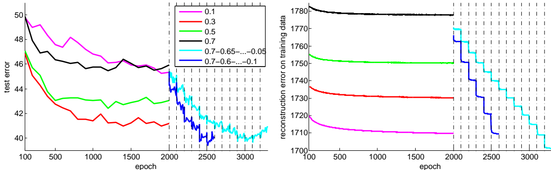
Figure 1: Experimental results with CIFAR-10 for 2000 hidden units. Test errors (left) and reconstruction error on training set (right) as a function of the number of epochs. Dashed lines indicate a point when the level of noise was changed. Test errors were measured every 100 training epochs initially (during the first 2000 epochs). After each change of the noise level, test error was measured after the first, the third, the fifth epoch and then after every ten epochs. Reconstruction errors were measured after each training epoch. For clarity, we do not show the results of DA (0.2), DA (0.4) and DA (0.6), which yield higher test error than DA (0.3).
